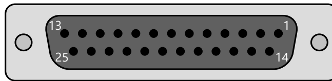
Figure 3: Female DB25 connector pin layout
