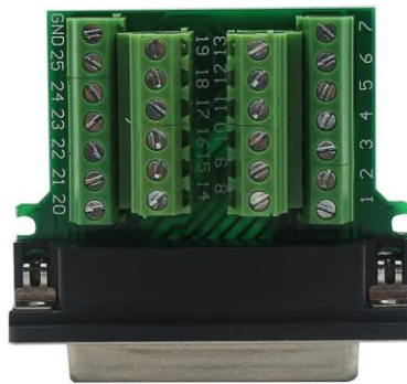
Figure 6: Male DB25 field splice connector pin layout
